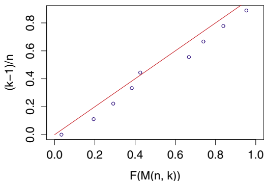
Fig. 30. GEV pp-plot of the maximal values of the exceptional snow loads in Region 2.
