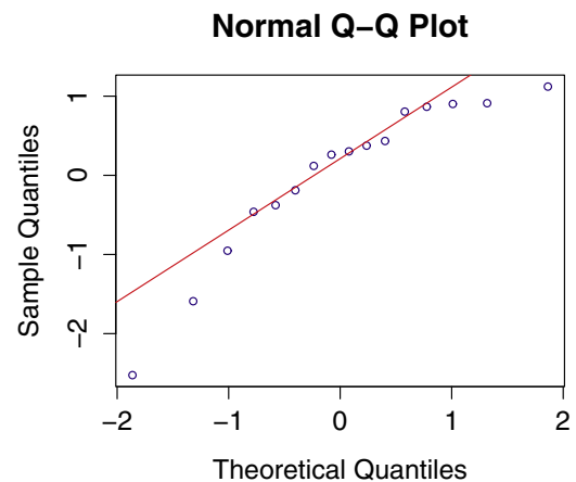
Fig. 17. Normal qq-plot of the error terms in model (21).
