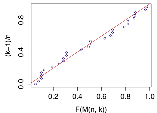
Fig. 9. GPD pp-plot of the maximal values of the exceptional snow loads in Region 1.
