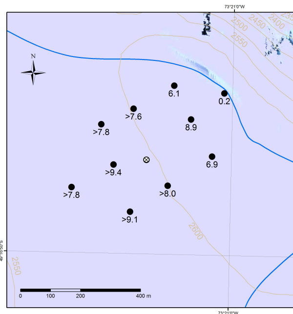
Fig. 7. Stake network (solid black circles) deployed around the drilling site (empty circle with x). The numbers at each stake represent snow accumulation in \text{cm day}^{-1} . The thick blue line shows the location of a prominent ridge which marks the ice divide between Pío XI Glacier and Viedma Glacier to the north and to the east. The brown lines are contour lines with elevations in m a.s.l., obtained from the SRTM 2000 data. All stakes located lower than 2600 m were lost due to snow burial, showing a snow accumulation larger than 7 \text{ cm day}^{-1} . At the highest stake, snow accumulation was practically zero, which is due to enhanced wind in the proximity of the ridge. The background image is a Quickbird scene of 26 December 2004, obtained from Google Earth, which shows a crevasse immediately northeast of the ridge, and some rock outcrops farther downslope.
