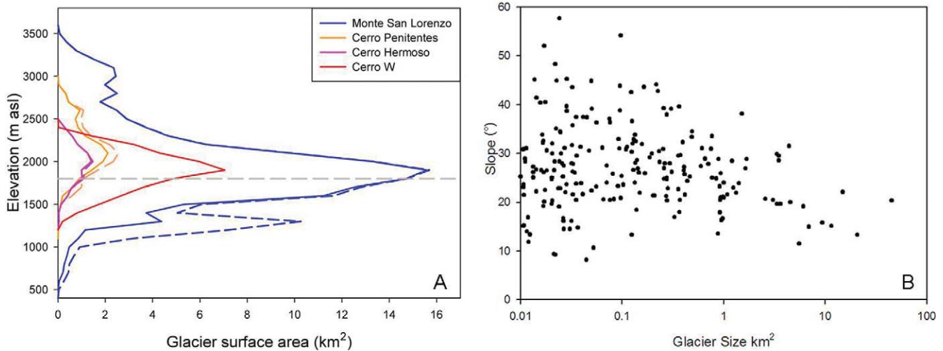
FIGURE 4. (A) Hypsometric distribution for the glaciated area in the Monte San Lorenzo region. The bare ice is represented by solid lines and the debris-covered portions in long dashed line. The horizontal dashed gray line indicates the ELA at 1800 m as reported by Wenzens (2002). (B) Variation of mean slope vs. glacier size; small ice bodies exhibit a broader scatter than larger glaciers.
